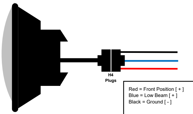
LED Replacement with H4 Plug
