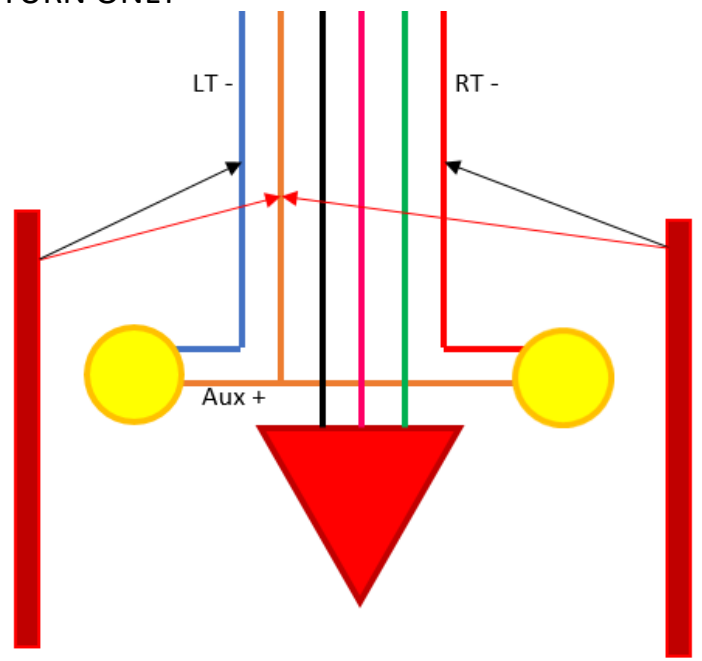
TURN ONLY
