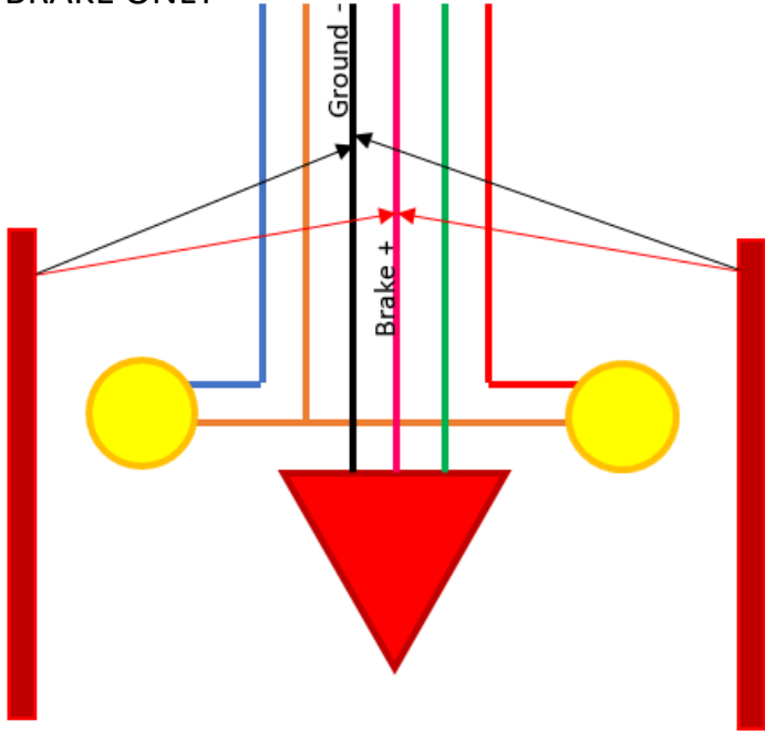
BRAKE ONLY
