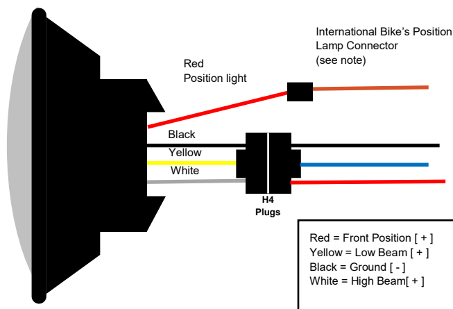
LED Replacement with H4 Plug
