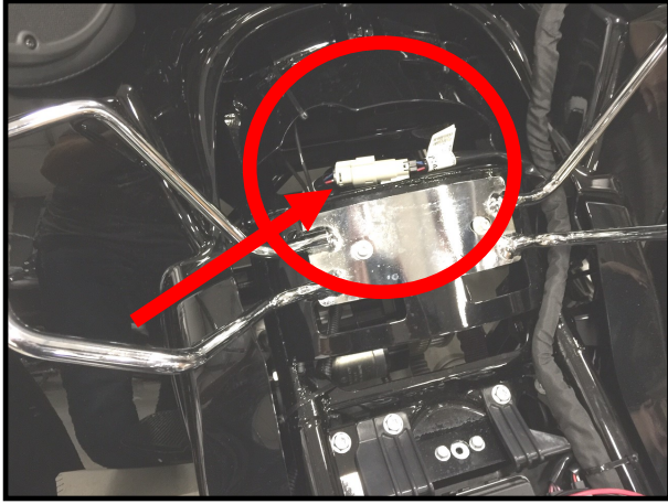
Trike Connector Location - Seat Removed
